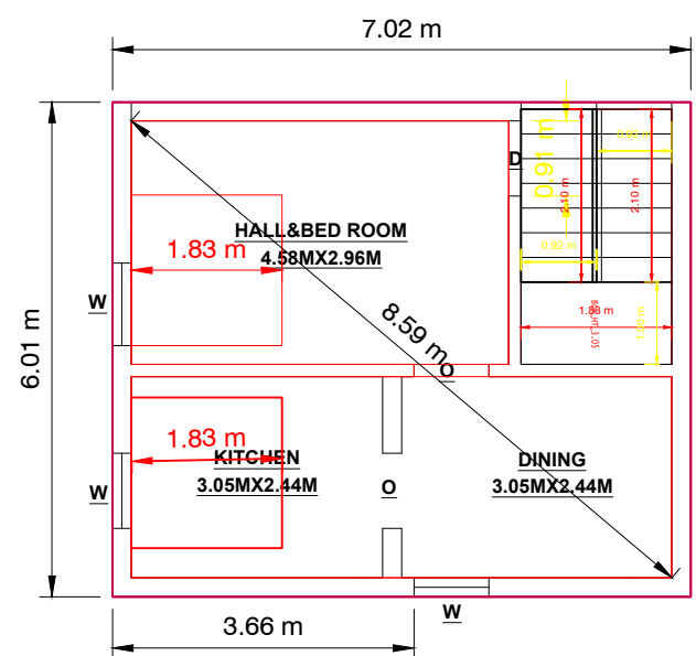
RESIDENTIAL FIRST FLOOR
