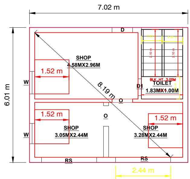
COMMERCIAL GROUND FLOOR
