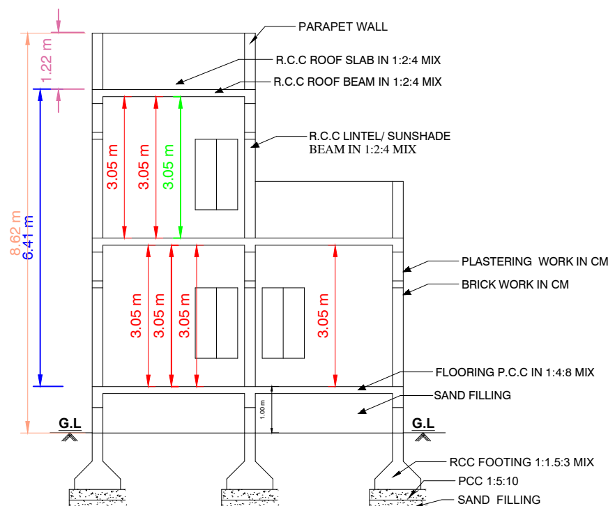
SECTION"AB"
