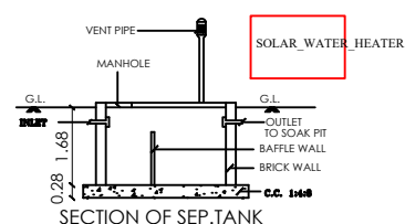
SECTION OF SEP.TANK
