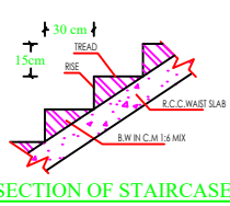
SECTION OF STAIRCASE
