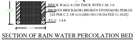
SECTION OF RAIN WATER PERCOLATION BED
