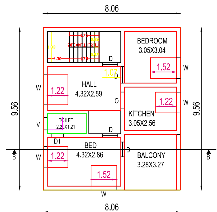
FIRST FLOOR PLAN ( PROPOSED BUILDING )
