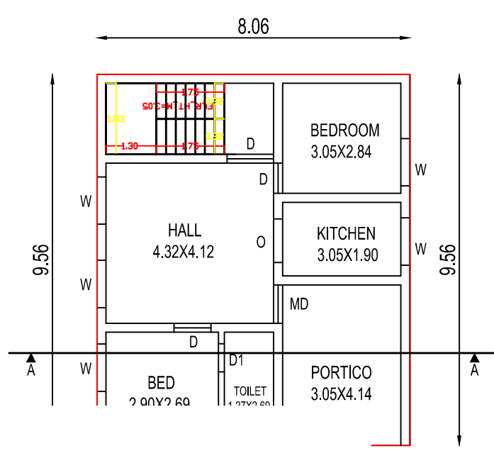
SECOND FLOOR PLAN ( PROPOSED BUILDING )
