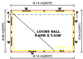
LOOMS BUILDING - PLAN
