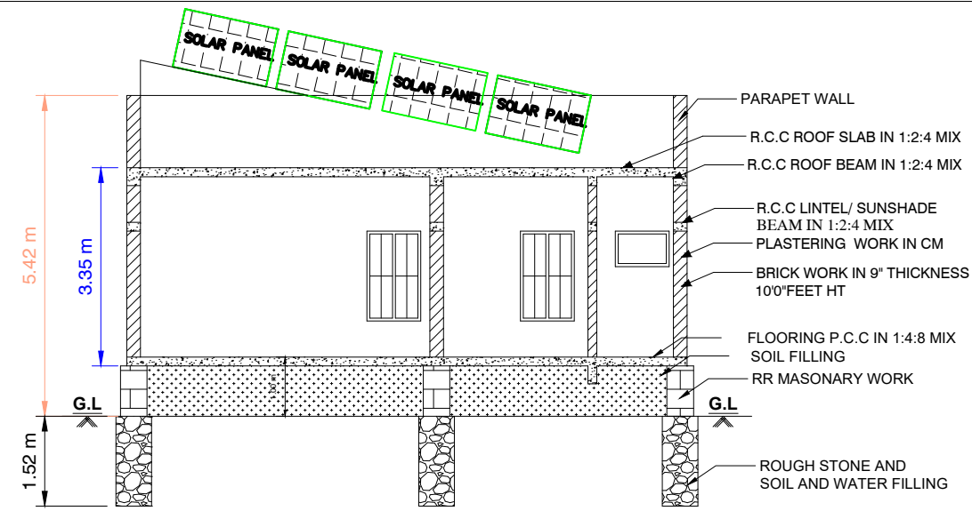
SECTION"AB"
