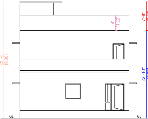
FRONT ELEVATION (EAST SIDE VIEW)
