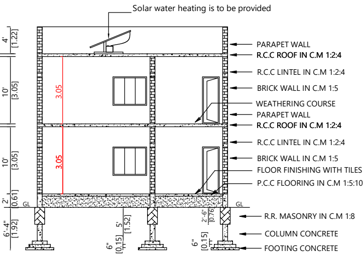
CROSS SECTION "AB"
