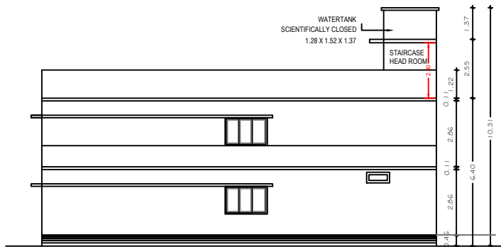
FRONT ELEVATION.
