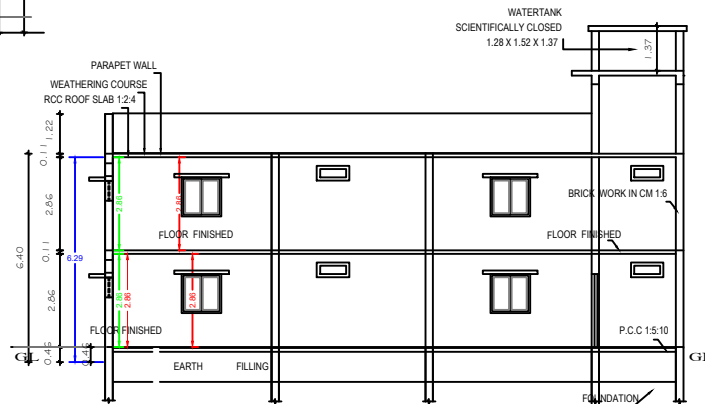
SECTION "A-B"
