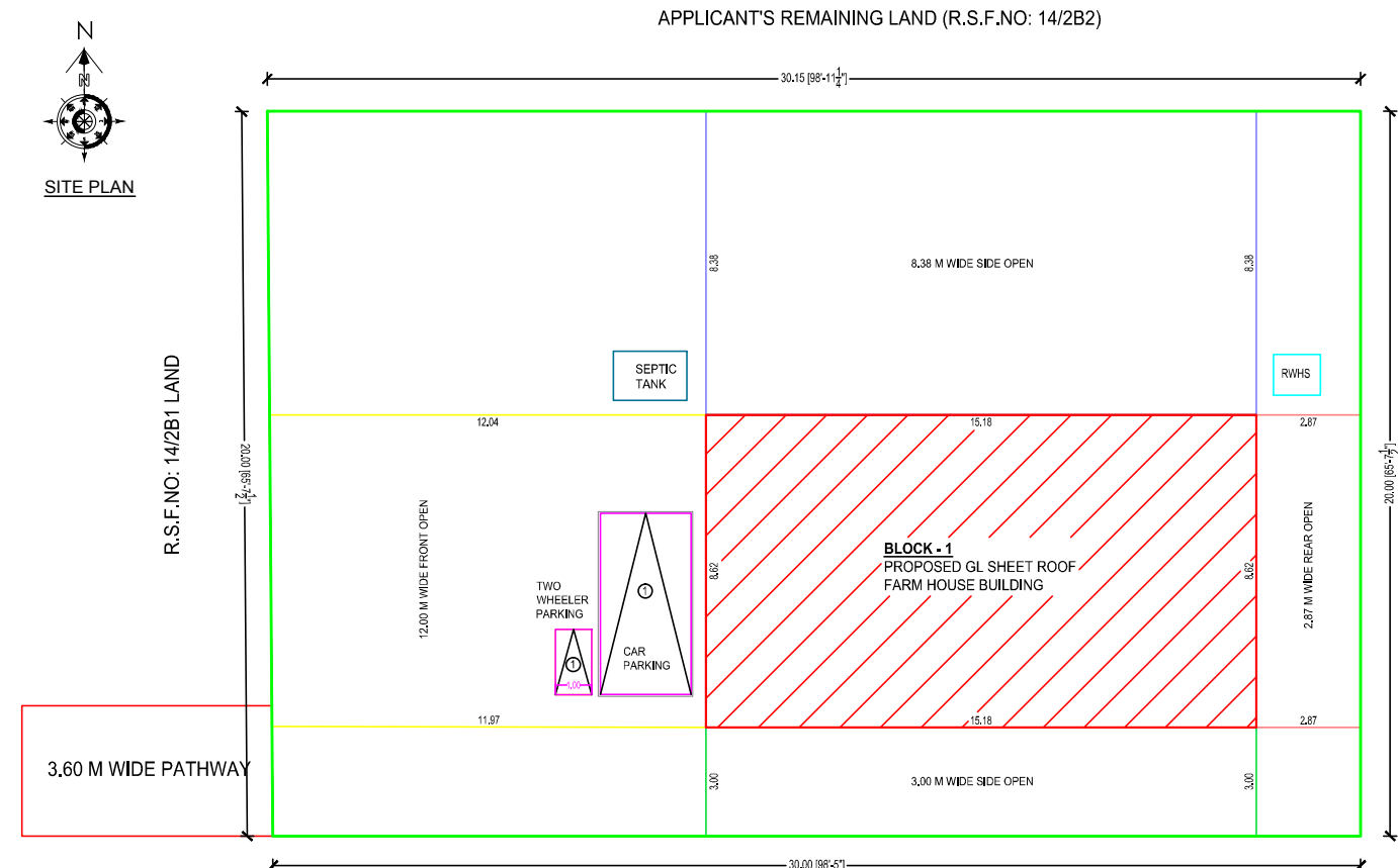
SITE PLAN
