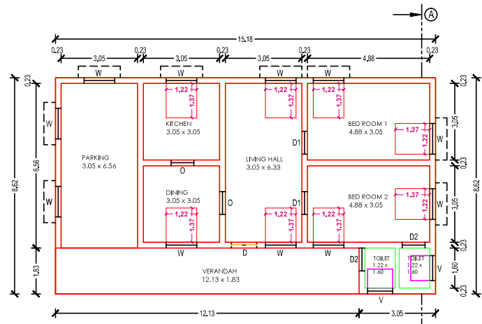
PLAN (PROPOSED FARM HOUSE BUILDING)
