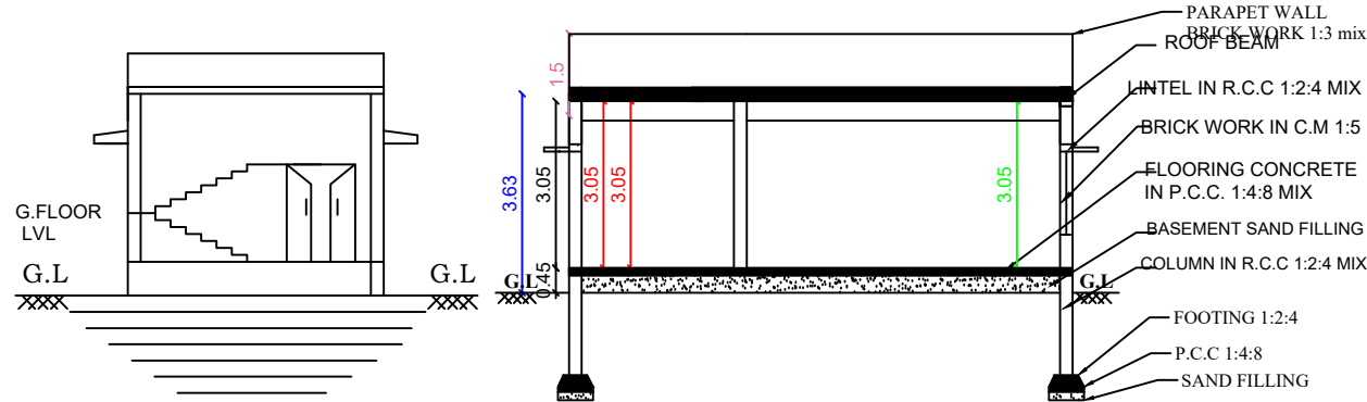
ELEVATION (East Facing)
