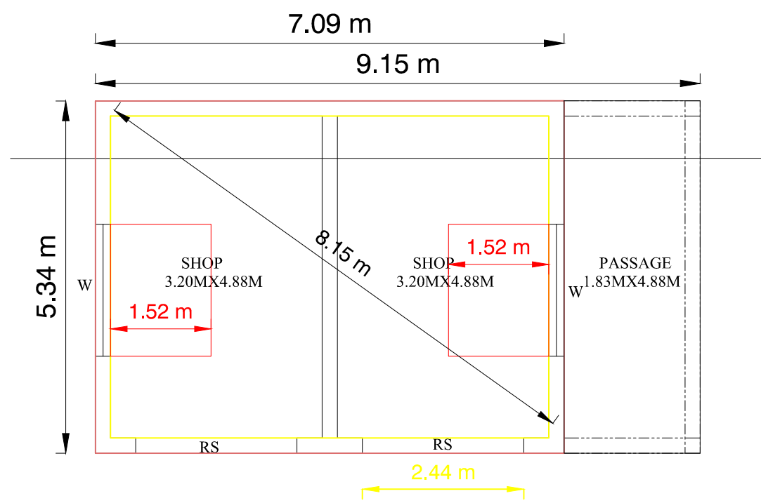
COMMERCIAL GROUND FLOOR
