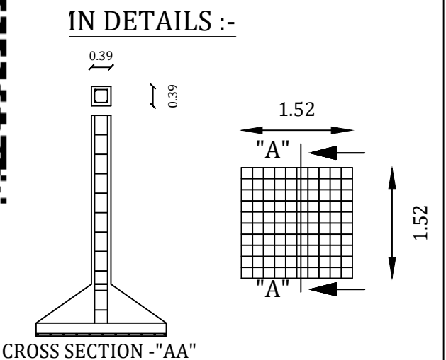
R PLAN
