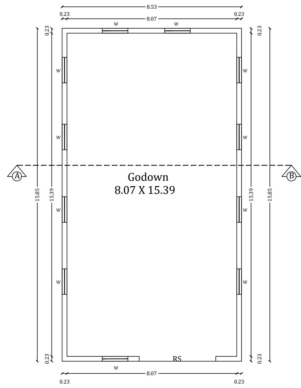
R PLAN
