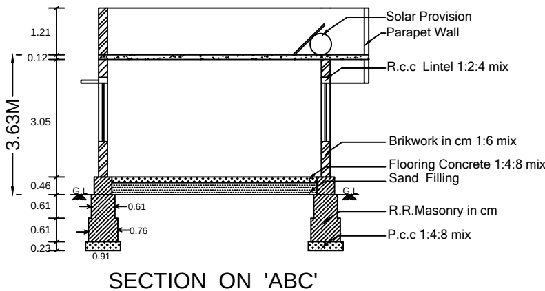
SECTION ON 'ABC'
