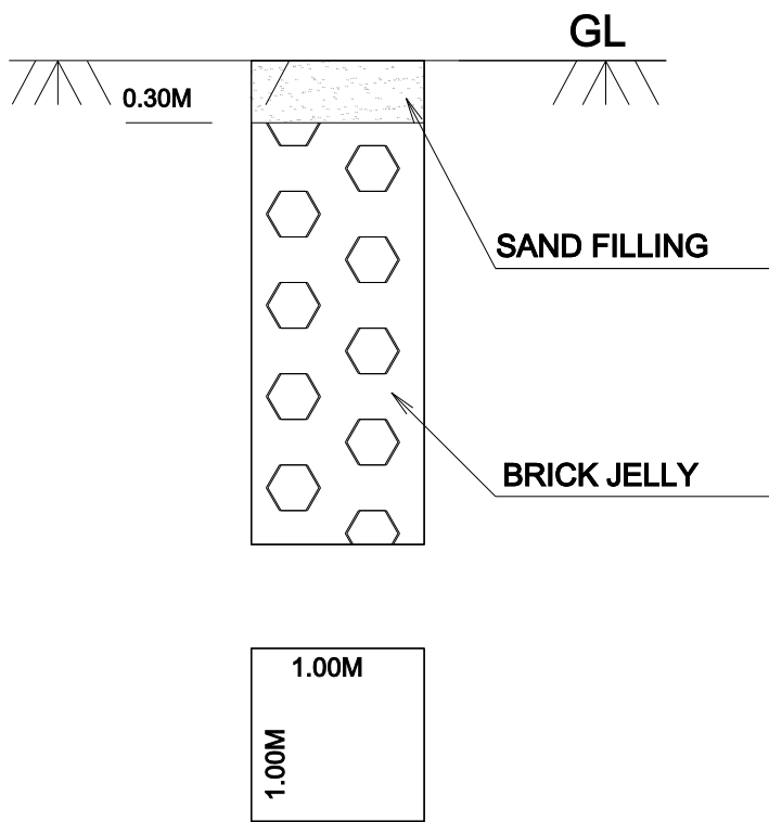
DETAILS OF RAINWATER HARVESTING TANK.(NTS)
