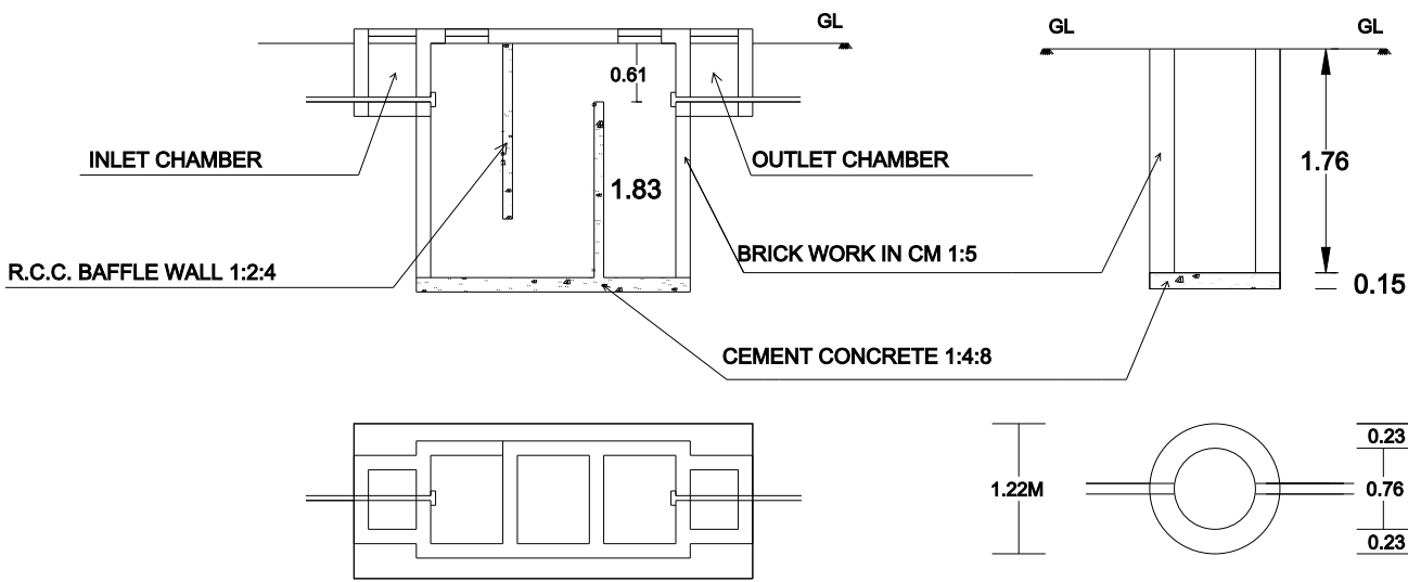
DETAILS OF SEPTIC TANK & SOAK PIT.
