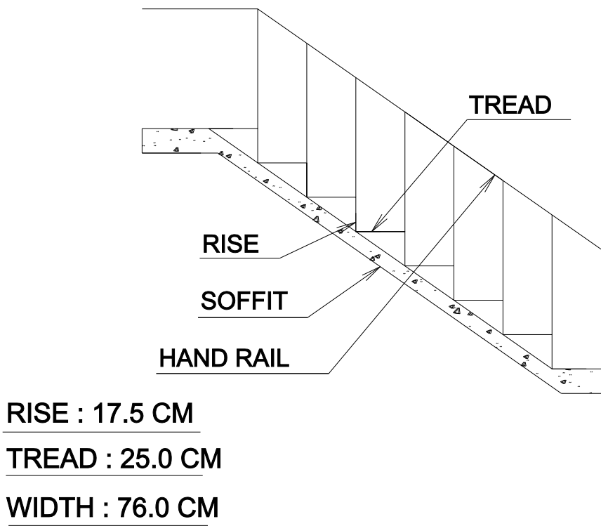
STAIRCASE DETAILS (NTS)
