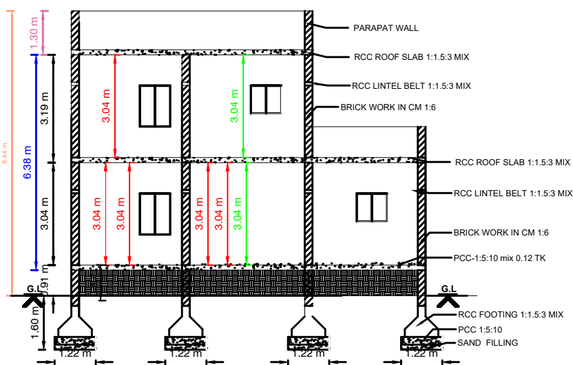
SECTION "AB"
