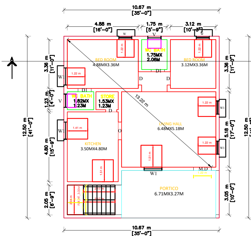
GROUND FLOOR PLAN ENTRANCE FACING TO EAST
