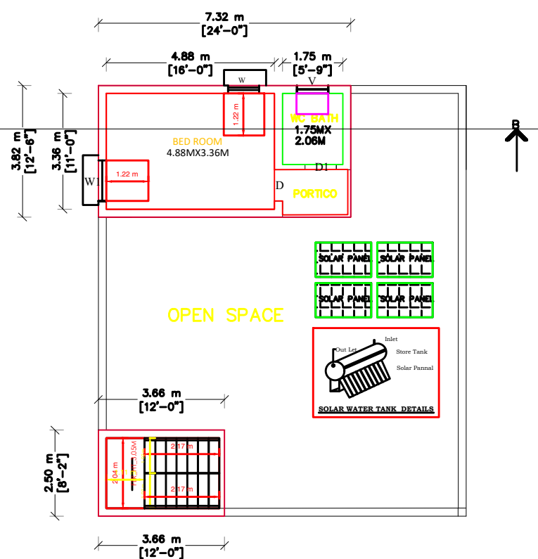
FIRST FLOOR PLAN ENTRANCE FACING TO EAST
