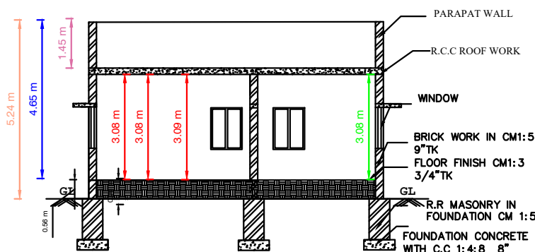
SECTION " AB "
