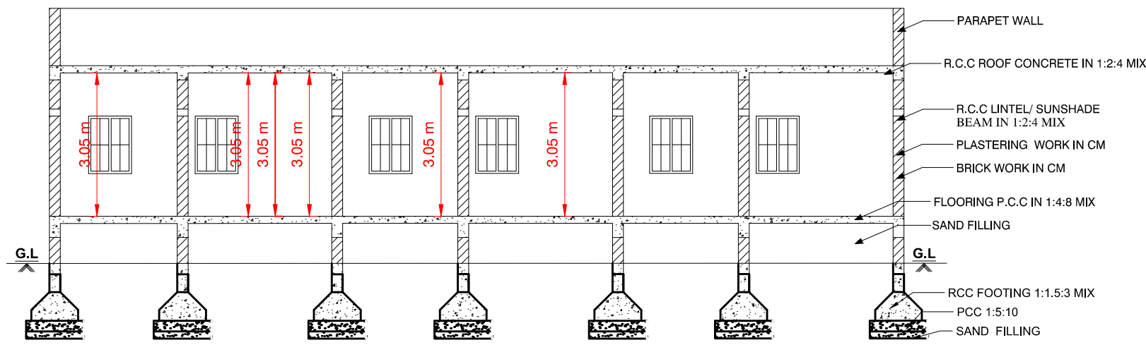
SECTION"AB"
