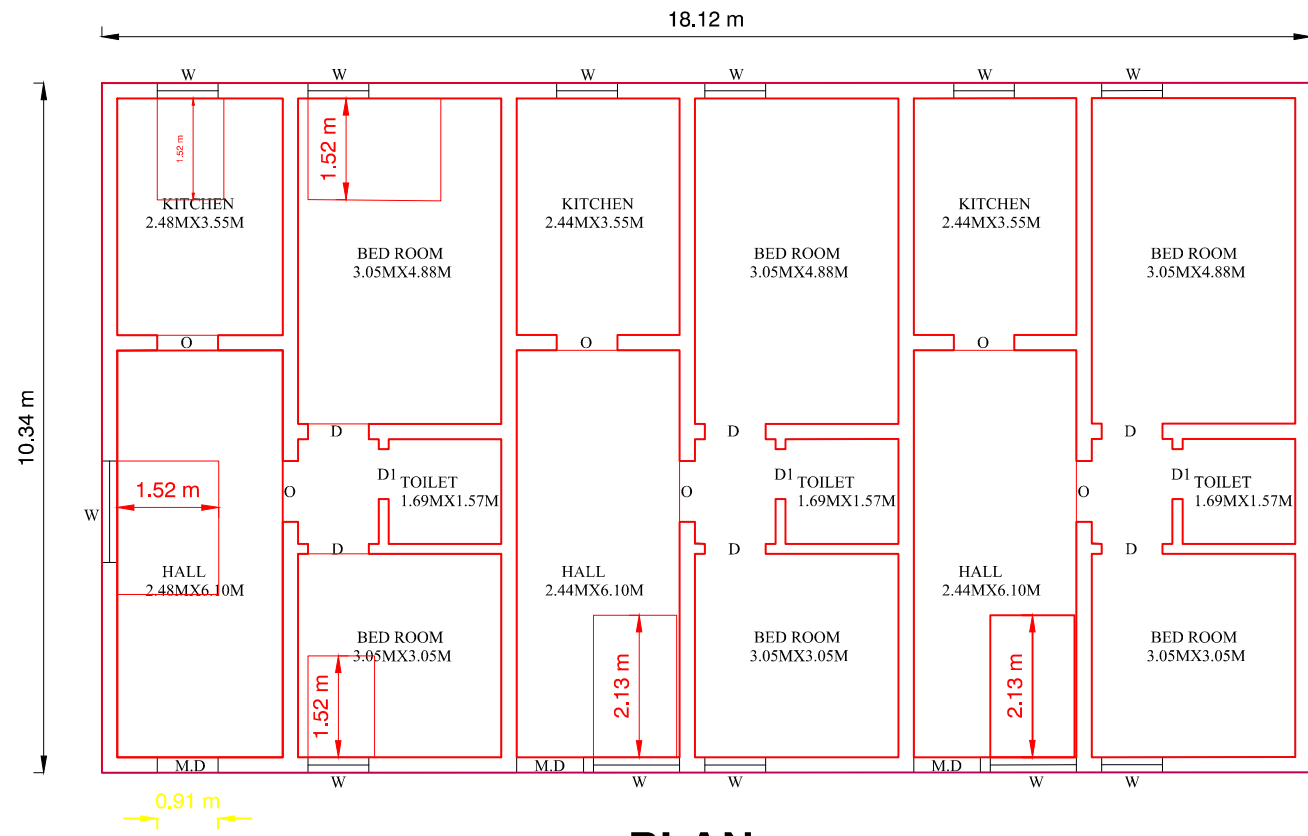
PLAN
