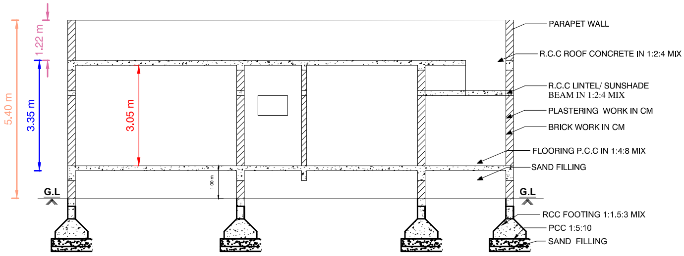
SECTION"AB"
