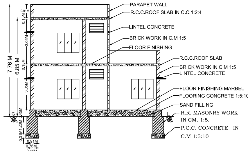
SECTION - XX
