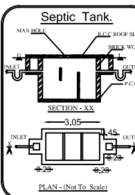
SECTION - XX
