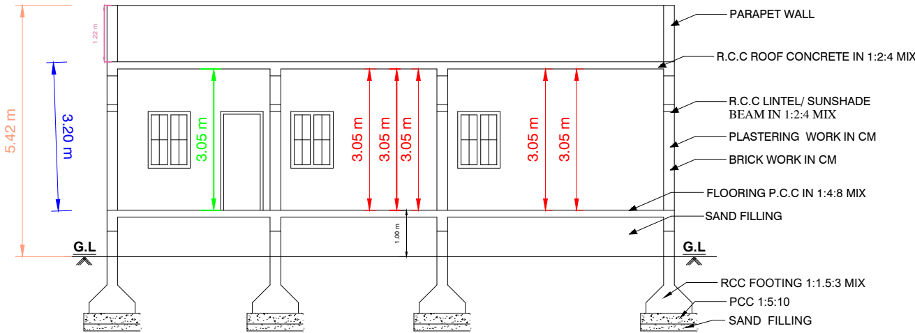
SECTION"AB"
