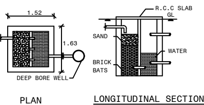
RAIN WATER HARVESTING FILTER BED
