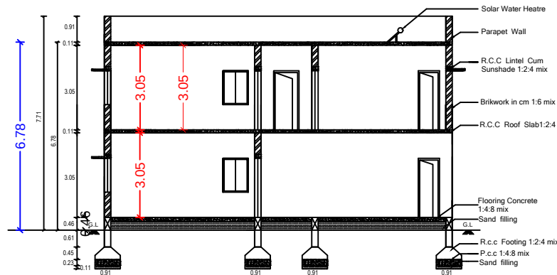
SECTION ON 'ABCD'
