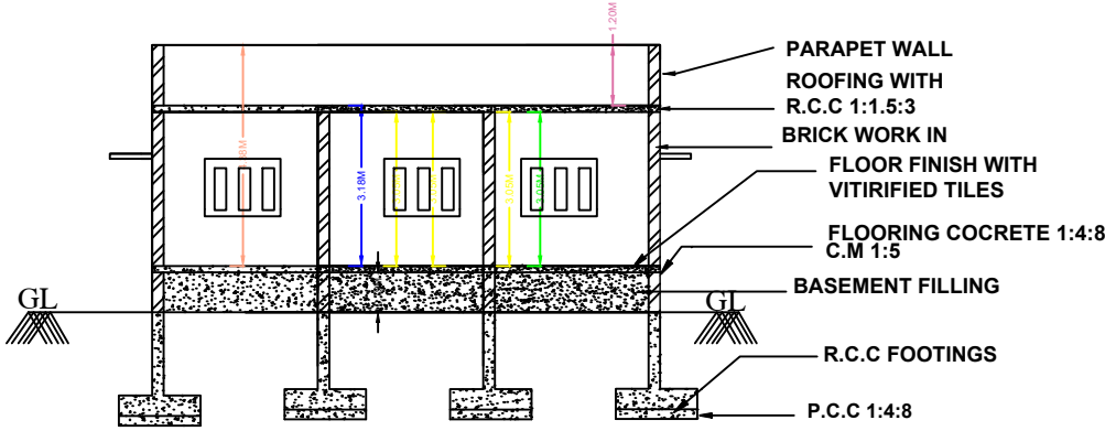
SECTION ON "BB1"
