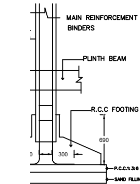
TYPICAL SECTION OF R.C.C. COLUMN FOUNDATION SCALE : 1" = 2'-0"
