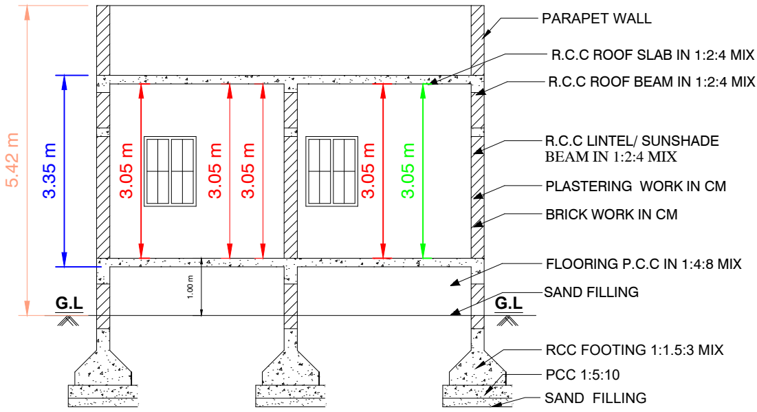
SECTION"AB"
