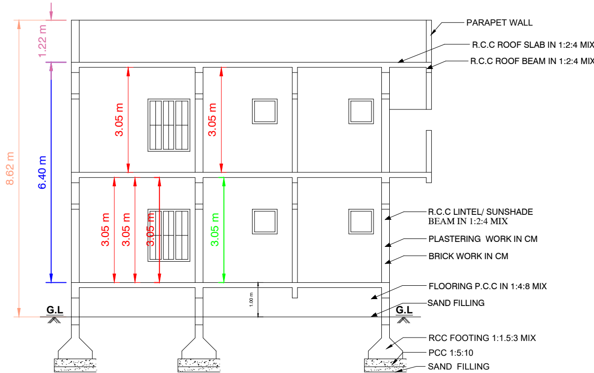
SECTION"AB"
