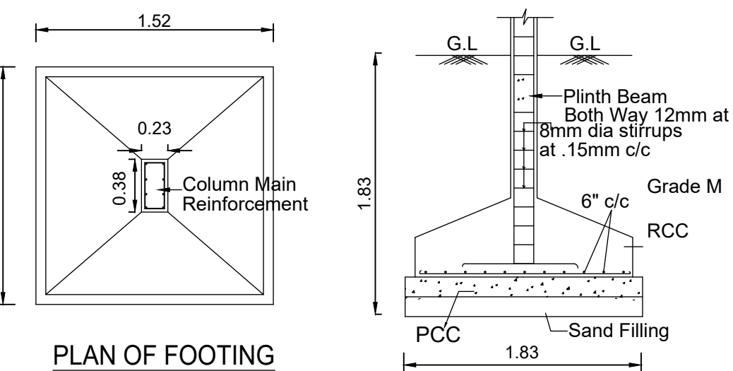
SECTION OF FOOTING
