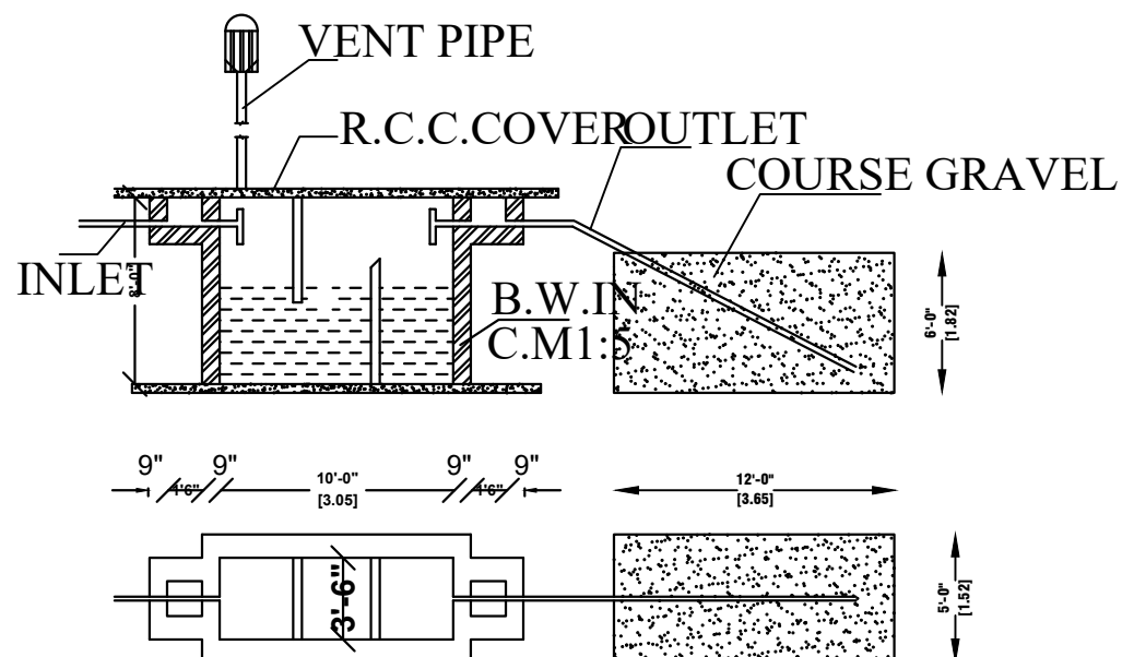
SEPTIC TANK & D-TRENCH DETAILS (NOT TO SCALE)
