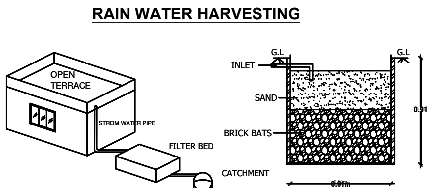
RAIN WATER HARVESTING
