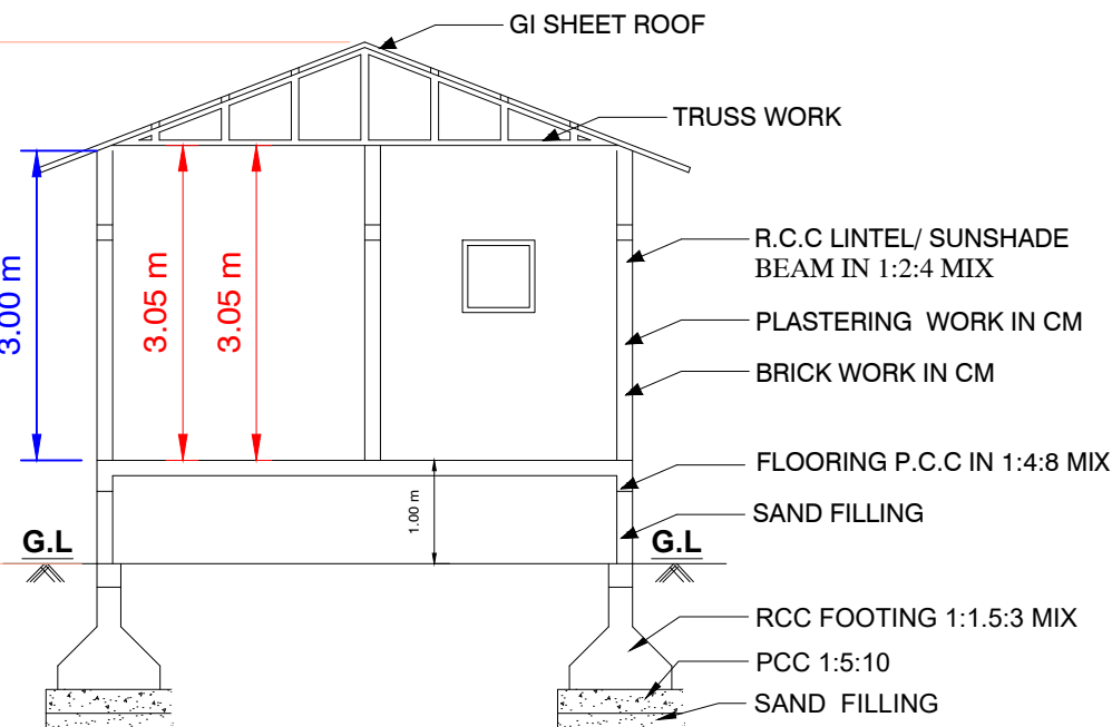
SECTION"AB"
