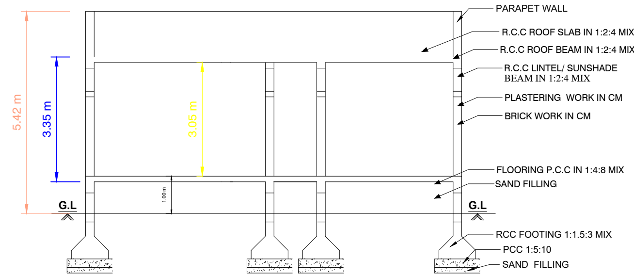
SECTION"AB"
