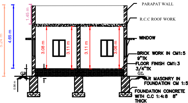
SECTION " AB "
