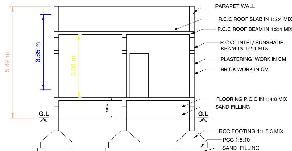
SECTION"AB"
