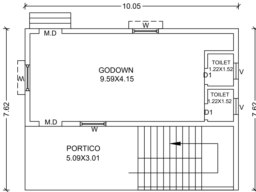
EXISTING APPROVED GROUND FLOOR PLAN
