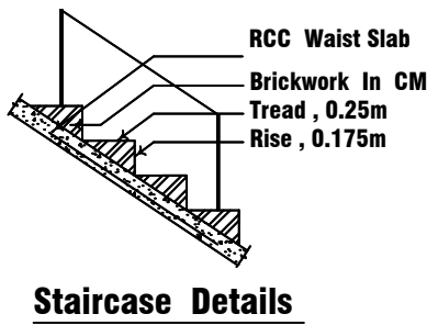
Staircase Details
