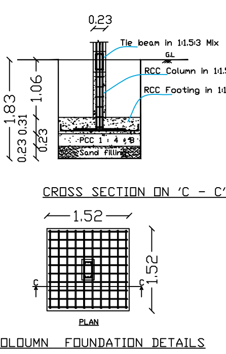
COLUMN FOUNDATION DETAILS
