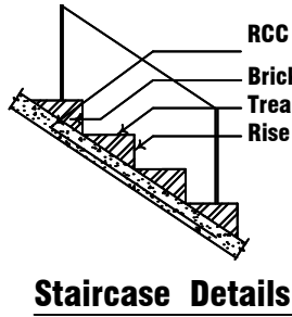
Staircase Details
