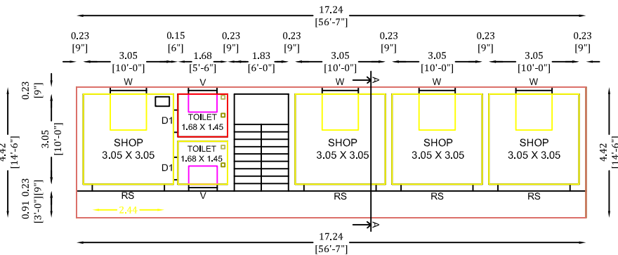
PLAN (SCALE-1:100)
