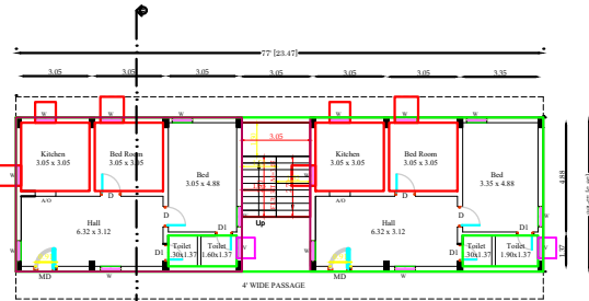
FIRST FLOOR PLAN SCALE - 1:100
