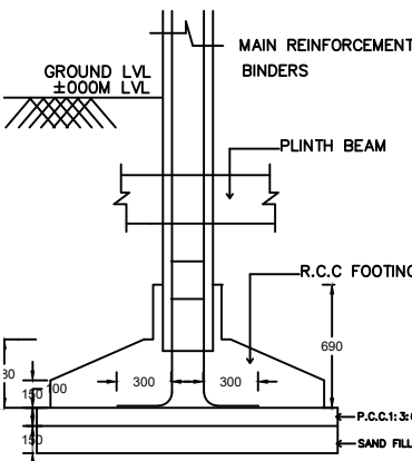
TYPICAL SECTION OF R.C.C. COLUMN FOUNDATION SCALE : 1" = 2'-0"
