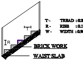
STAIRCASE & ENTRANCE STEPS
