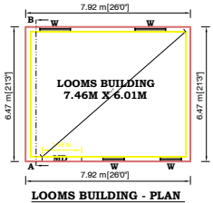
LOOMS BUILDING - PLAN
