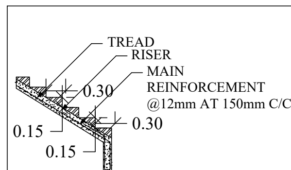
STAIRCASE DETAILS
