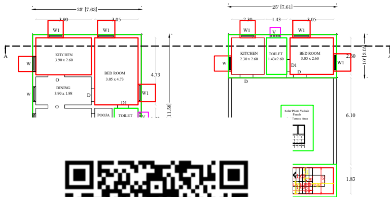
FLOOR PLAN S.F.NO: 282 - REMAINING LAND & AYANAR - LAND
