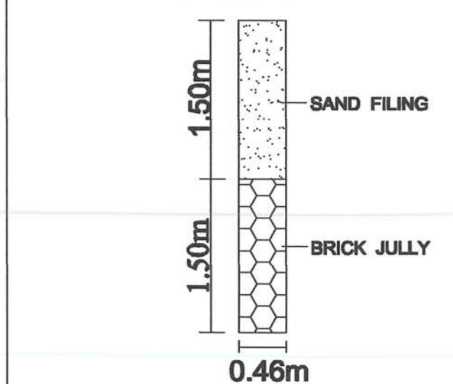
RAIN WATER PERCUSSION PIT
