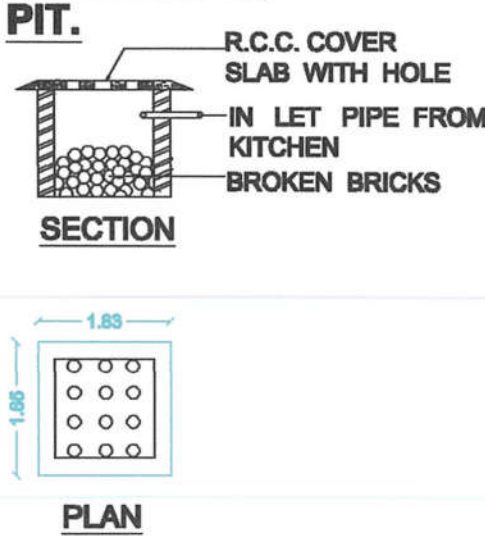
RAIN WATER HARVESTING PIT.
