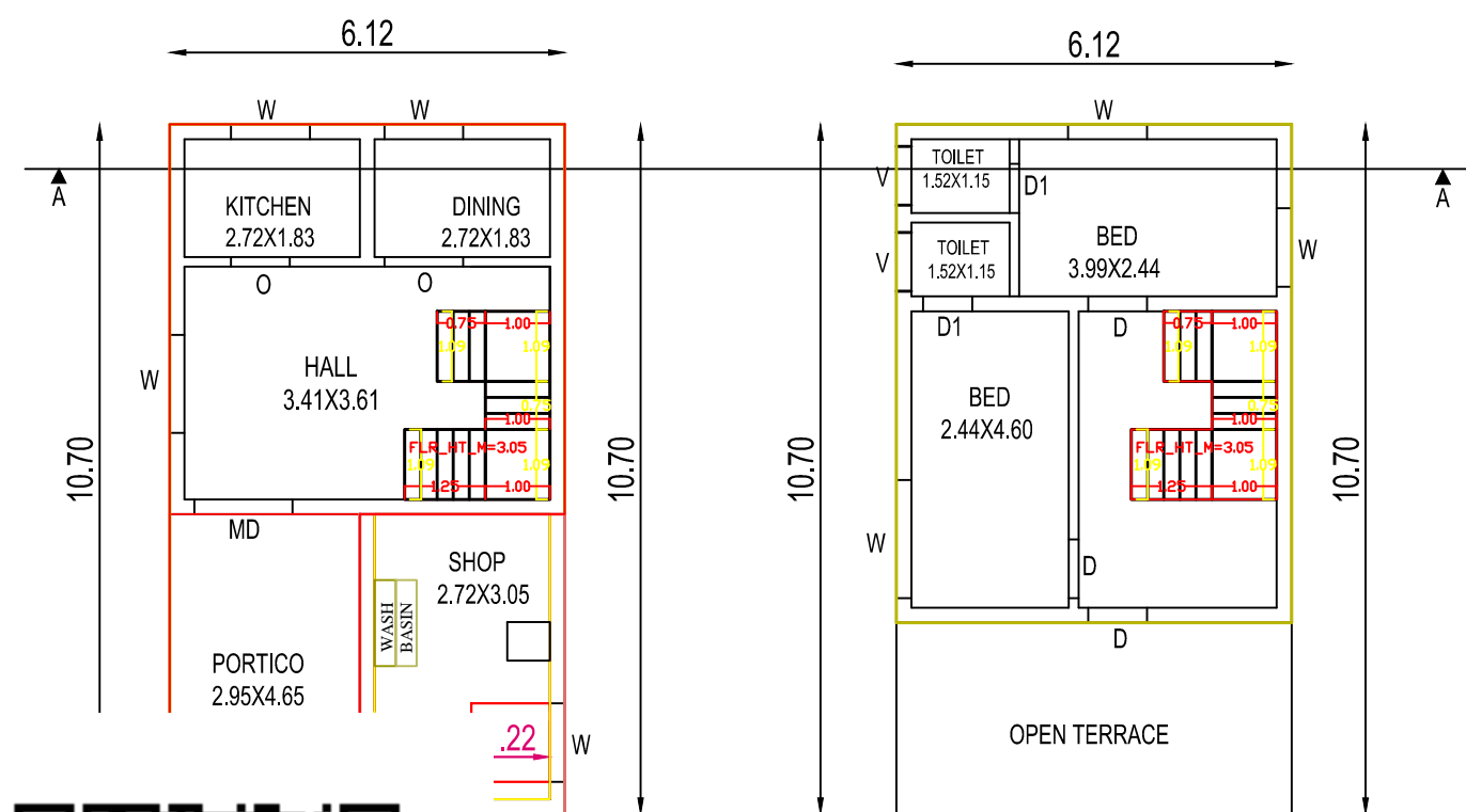
PLAN PROPOSED
