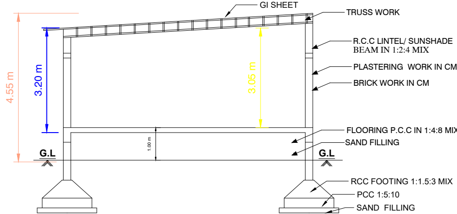
SECTION "AB"
