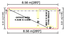
COMMERCIAL - PLAN
