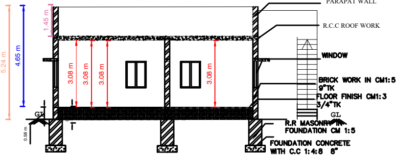
SECTION " AB "
