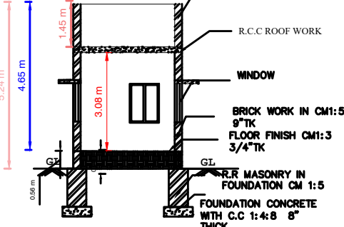
SECTION " AB "
