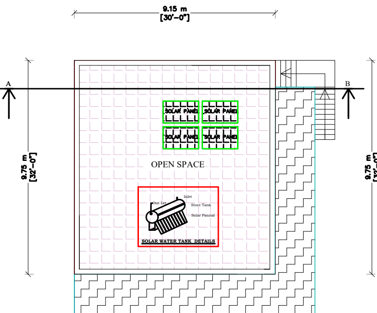
TERRACE PLAN
