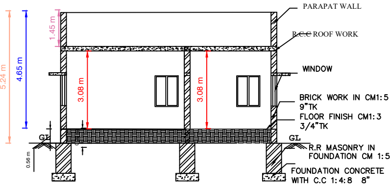
SECTION " AB "
