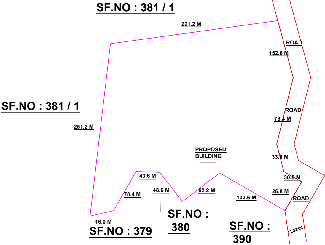
TOPO PLAN :
