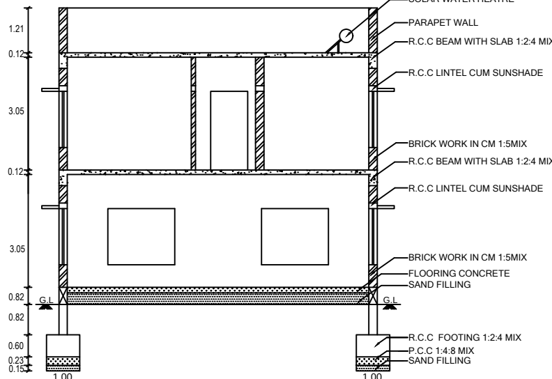
SECTION ON 'ABCD'
