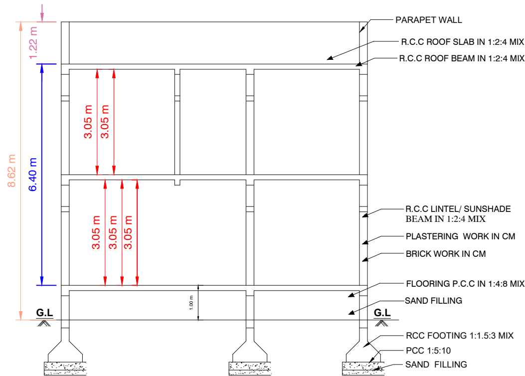
SECTION"AB"
