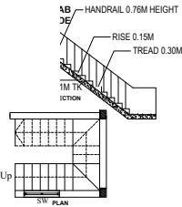
SW PLAN
