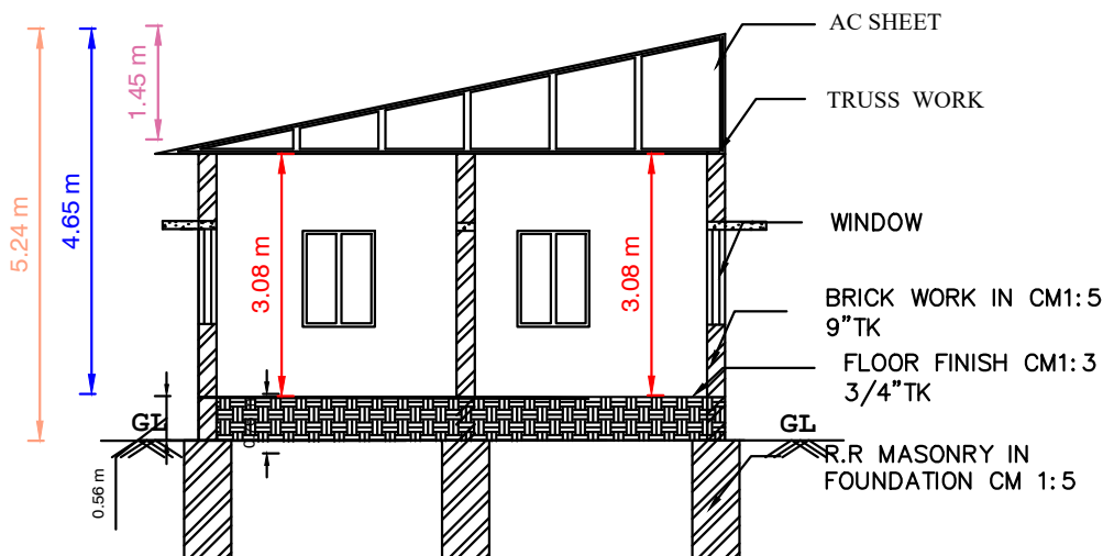
SECTION " AB "
