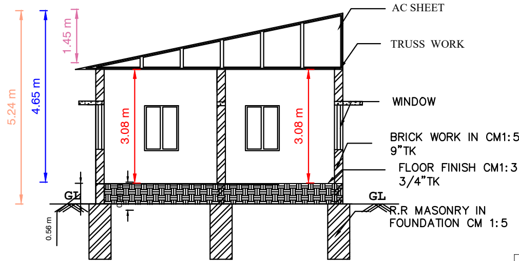
SECTION " AB "
