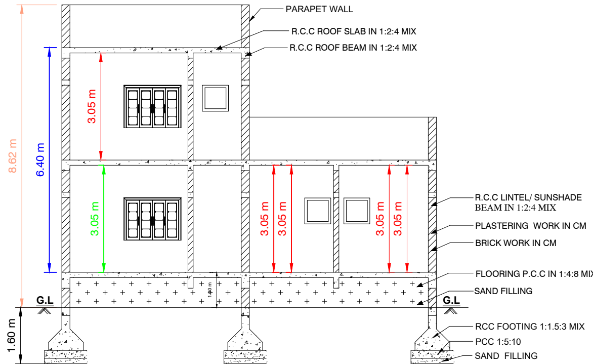
SECTION"AB"
